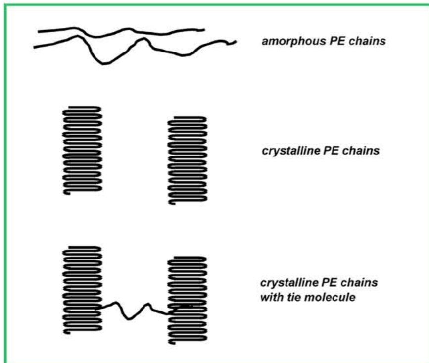
Fig 1: PE Chain Arrangements
